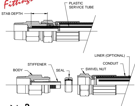
STAB DEPTH/STIFFENER CHART
